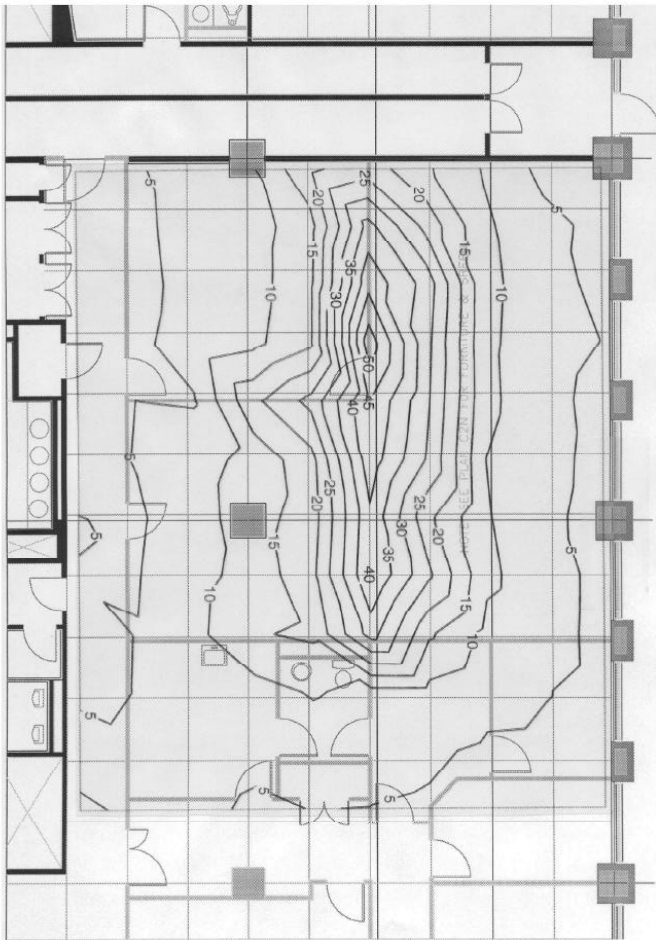
C1 Area - ELF EMI Levels in mGauss at 1 meter from floor slab.
